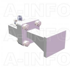
LB-51-10-C-SFSP Standard Gain Horn Antenna 15-22GHz 10dB Gain SMA Female
